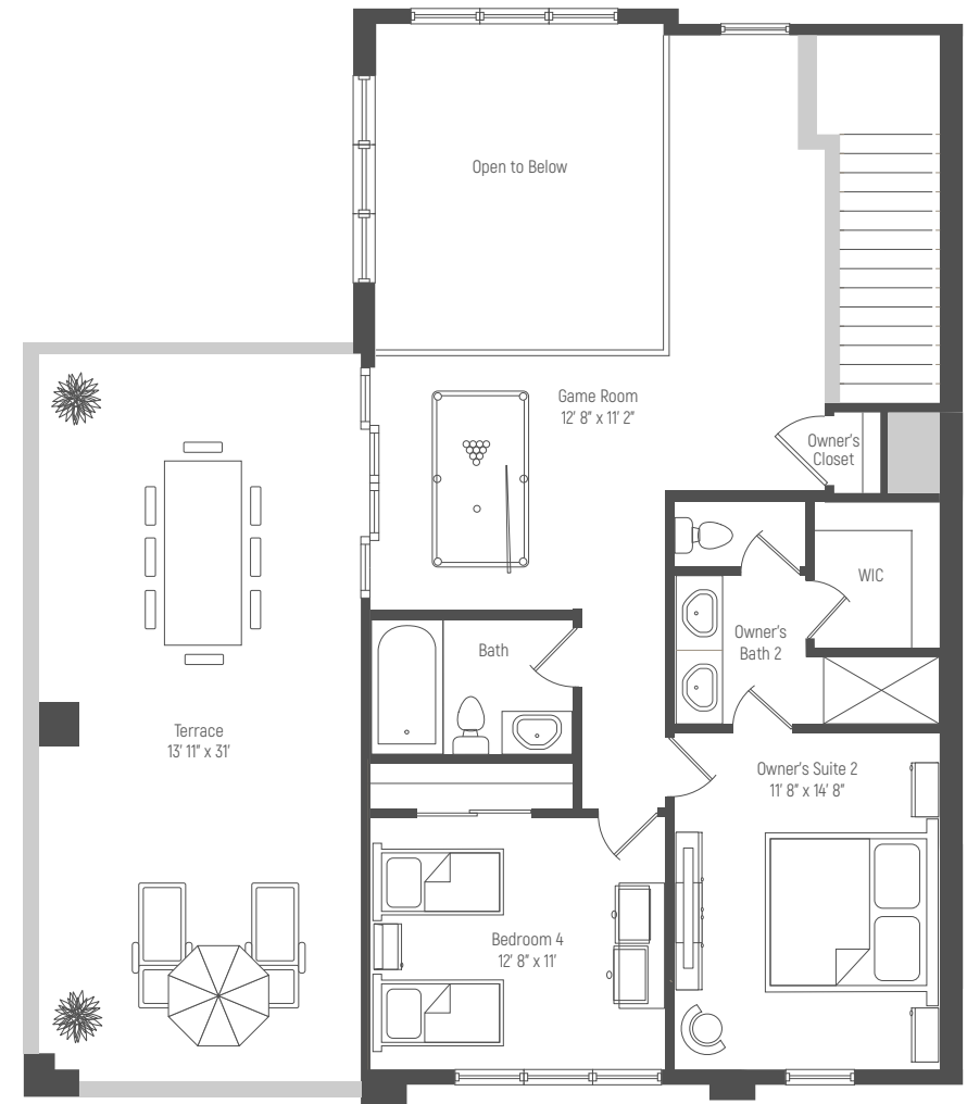
Upper Level
